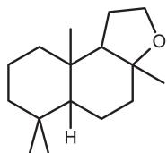
Naphtho[2,1-b]furan, dodecahydro-3a,6,6,9a-tetramethyl-
